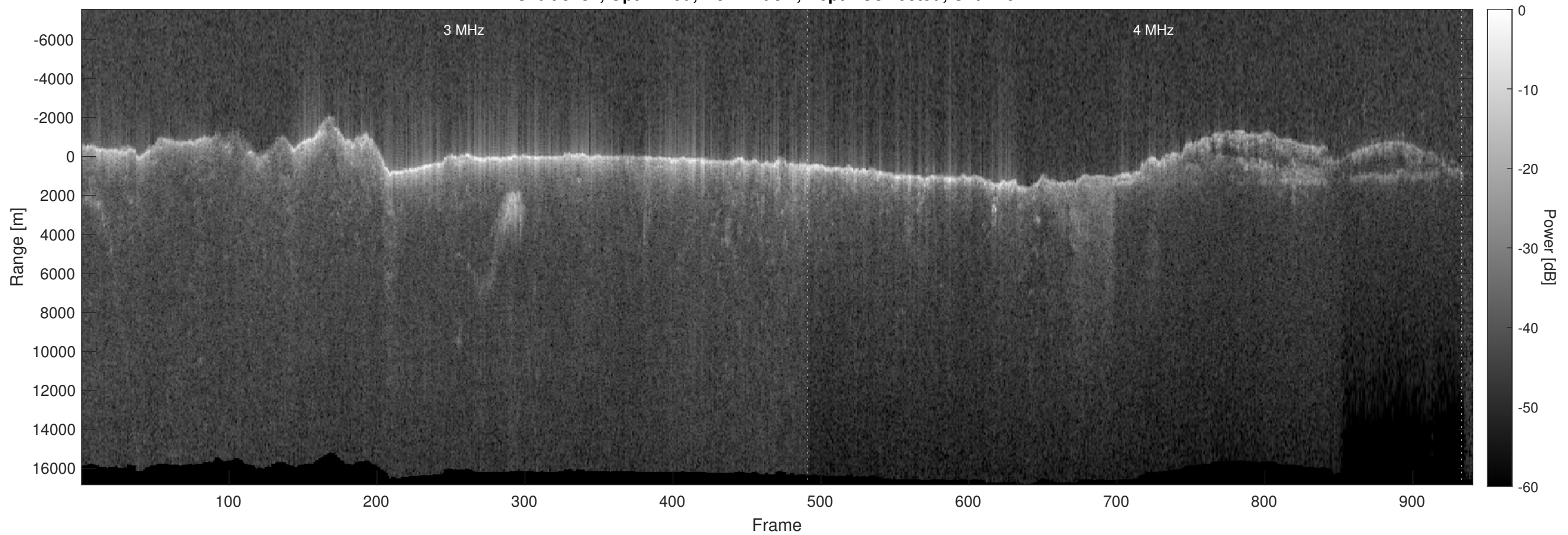
Orbit 5731, Optimized, No Window, Depth-Corrected, Channel 2
