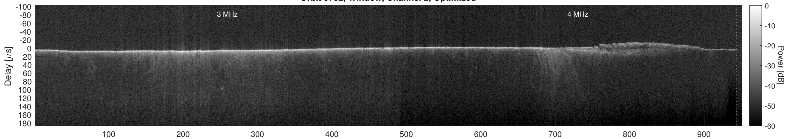
Orbit 5732, Cluttergram
