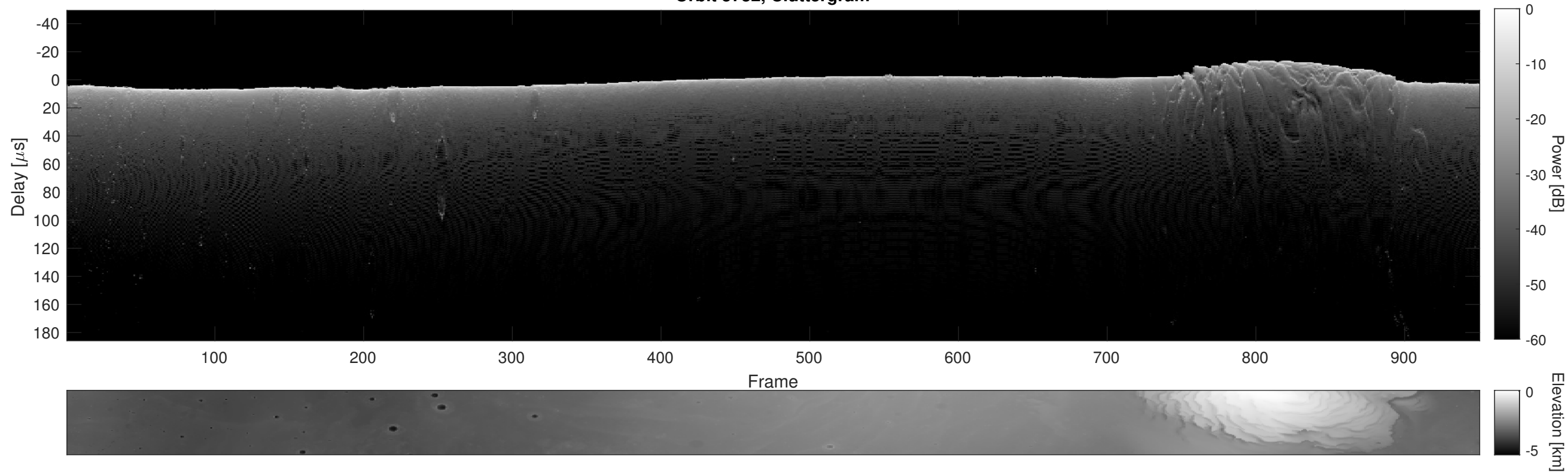
Orbit 5732, Cluttergram
