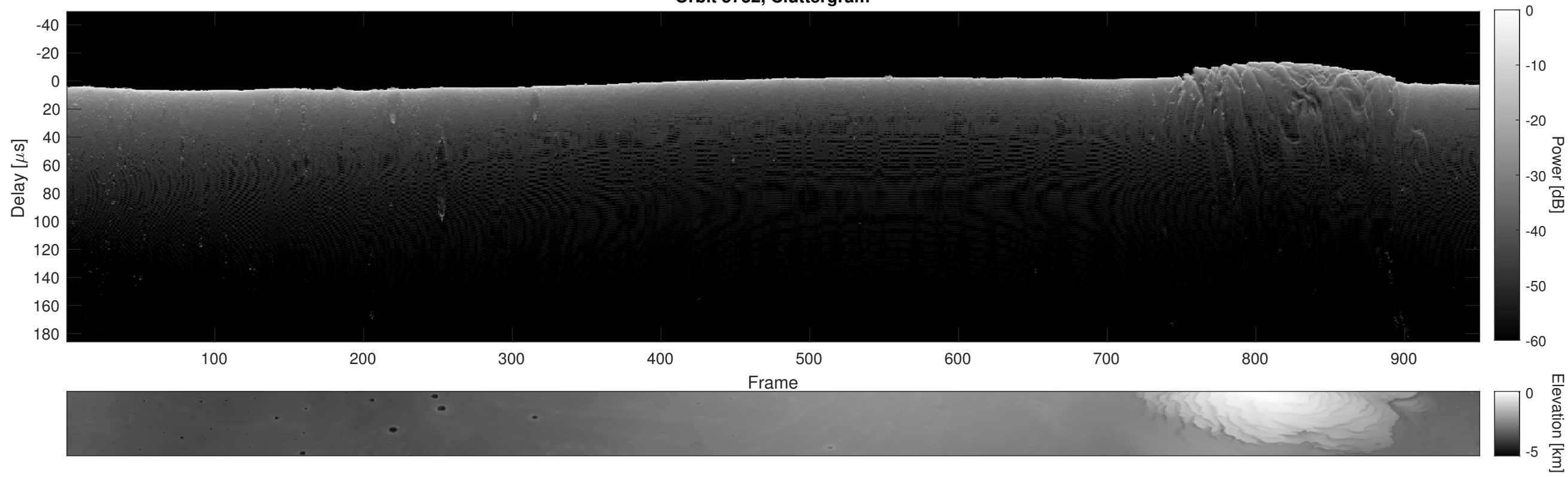
Orbit 5732, Cluttergram
