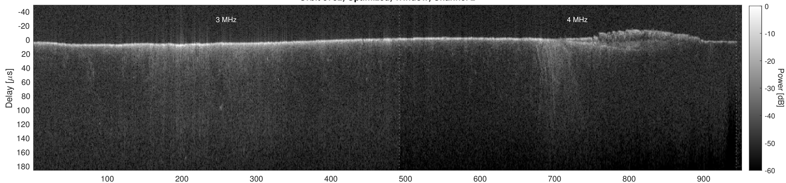
Orbit 5732, Cluttergram
