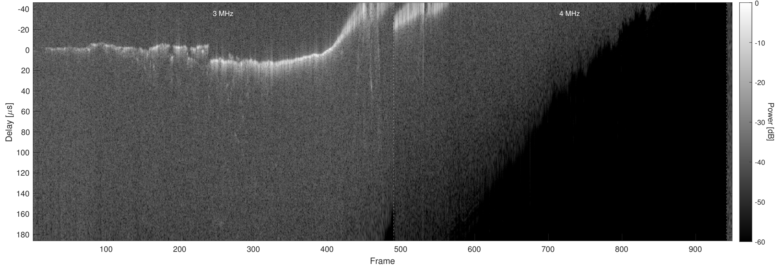
Orbit 5733, Chapman, No Window, Channel 2
