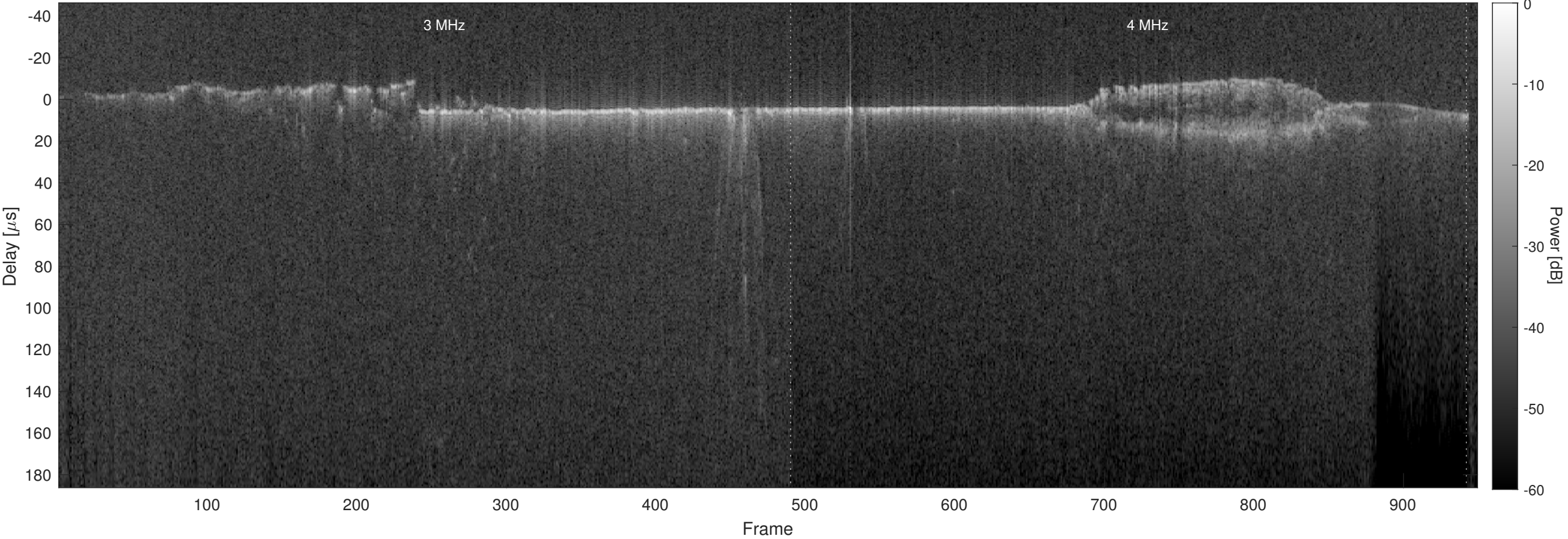
Orbit 5733, Optimized, No Window, Channel 2
