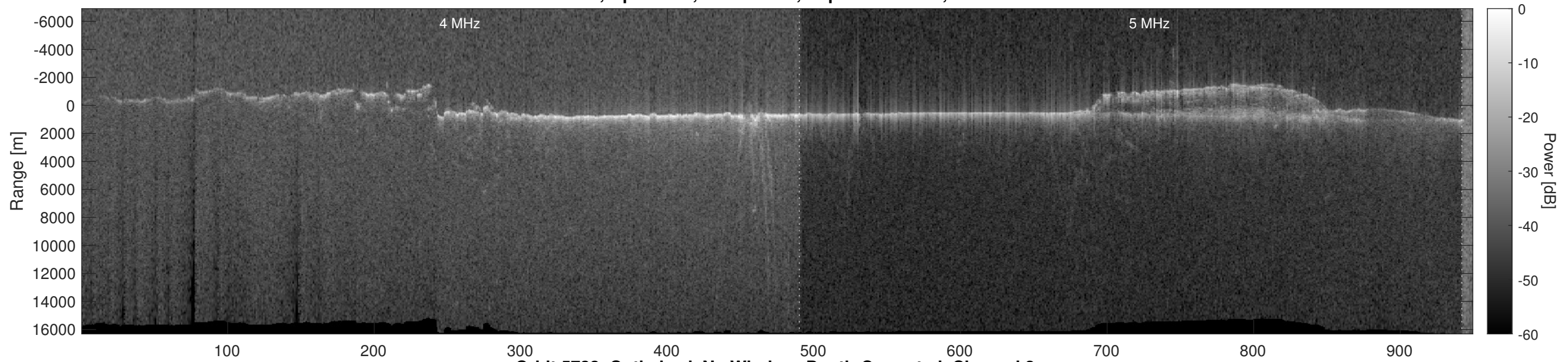
Orbit 5733, Optimized, No Window, Depth-Corrected, Channel 2
