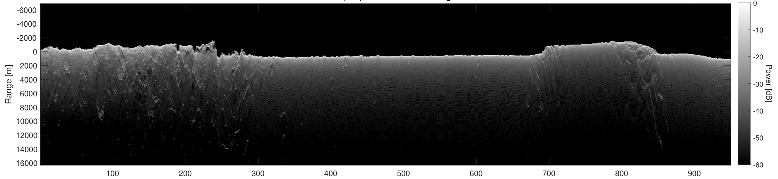
Orbit 5733, Depth-Corrected Cluttergram
