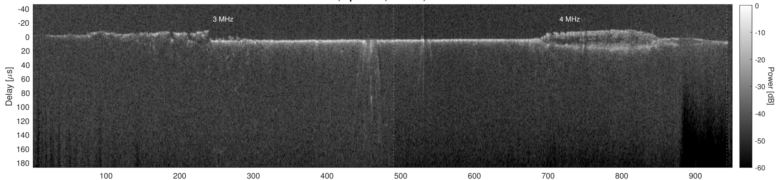
Orbit 5733, Cluttergram
