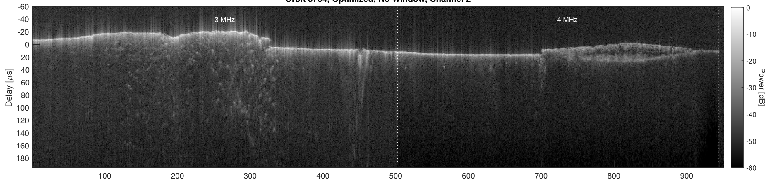
Orbit 5734, Cluttergram
