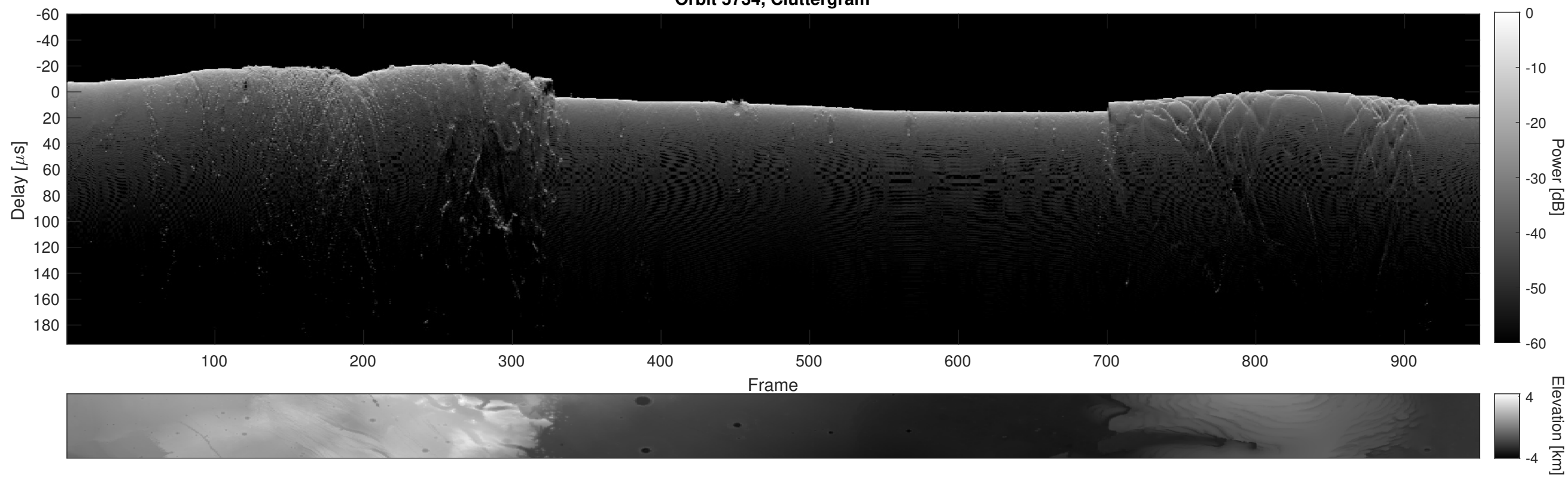
Orbit 5734, Cluttergram
