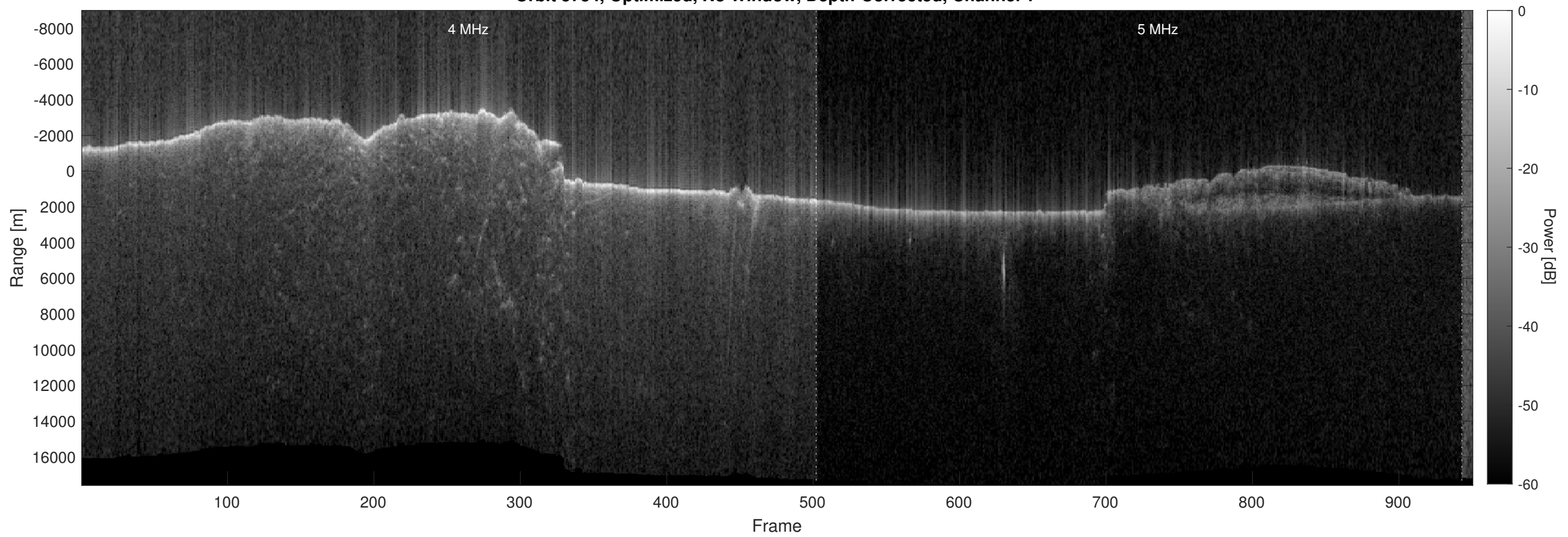
Orbit 5734, Optimized, No Window, Depth-Corrected, Channel 2
