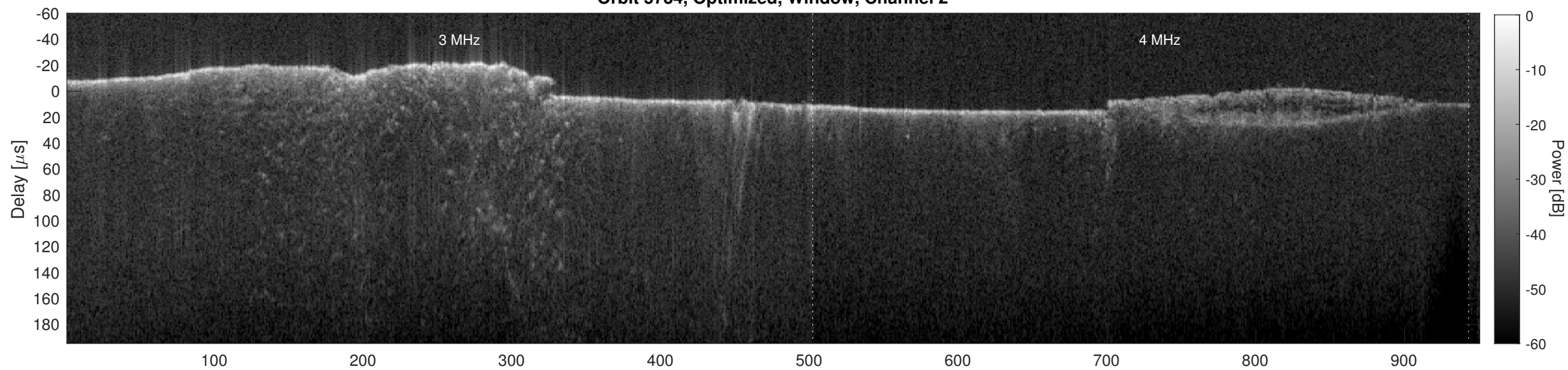
Orbit 5734, Cluttergram
