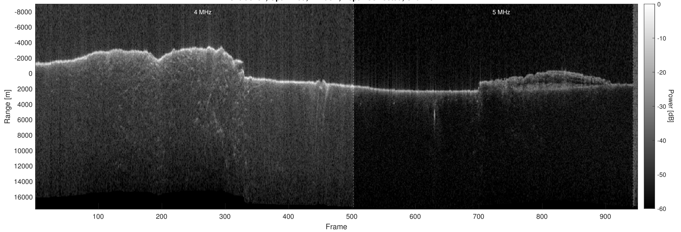
Orbit 5734, Optimized, Window, Depth-Corrected, Channel 2
