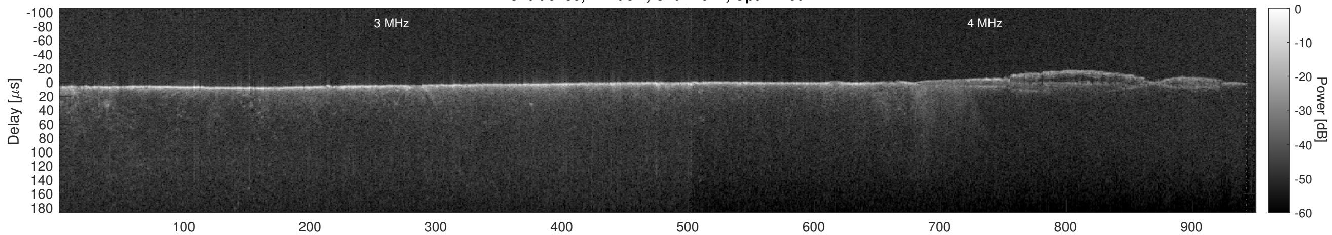
Orbit 5735, Cluttergram
