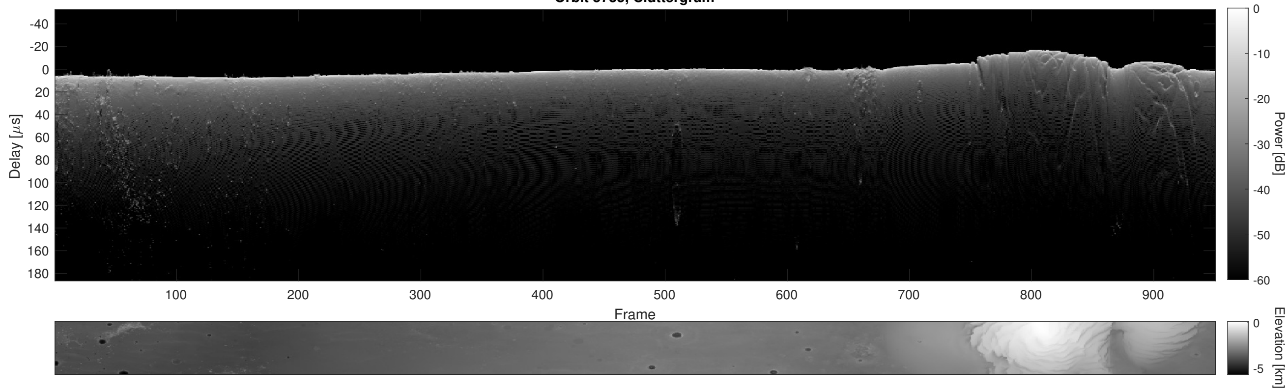
Orbit 5735, Cluttergram
