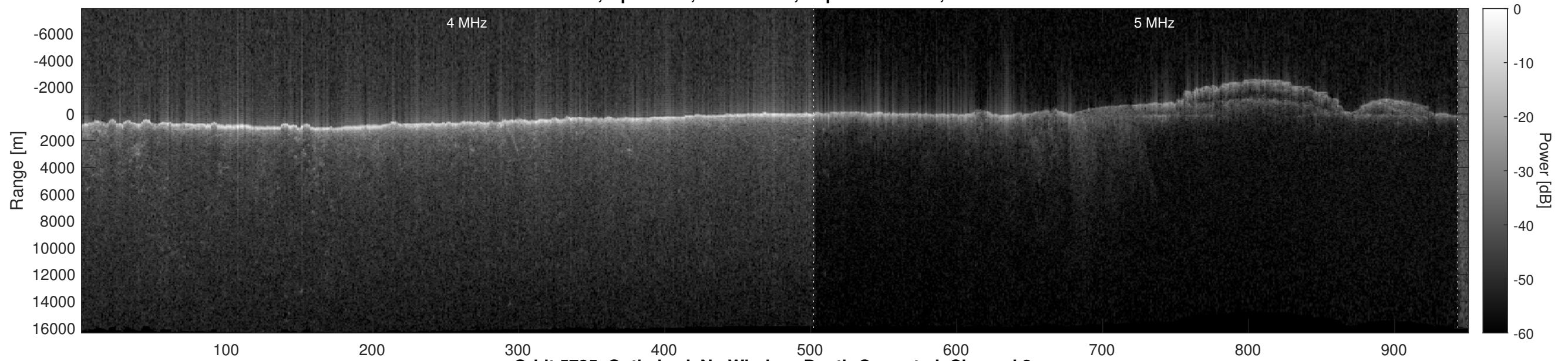
Orbit 5735, Optimized, No Window, Depth-Corrected, Channel 2
