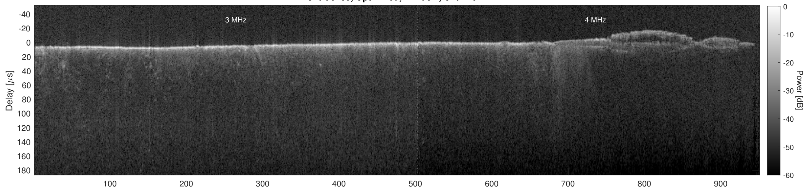
Orbit 5735, Cluttergram
