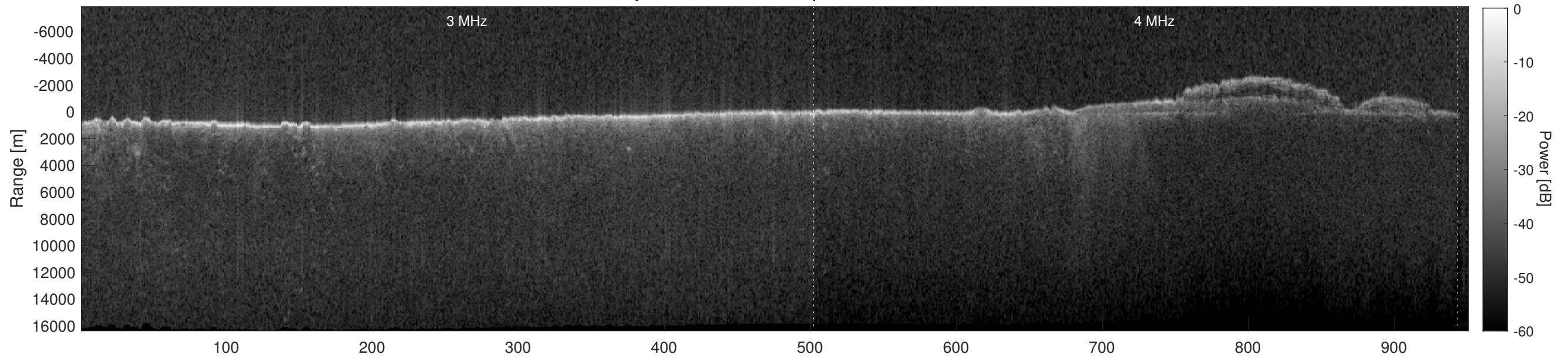
Orbit 5735, Depth-Corrected Cluttergram
