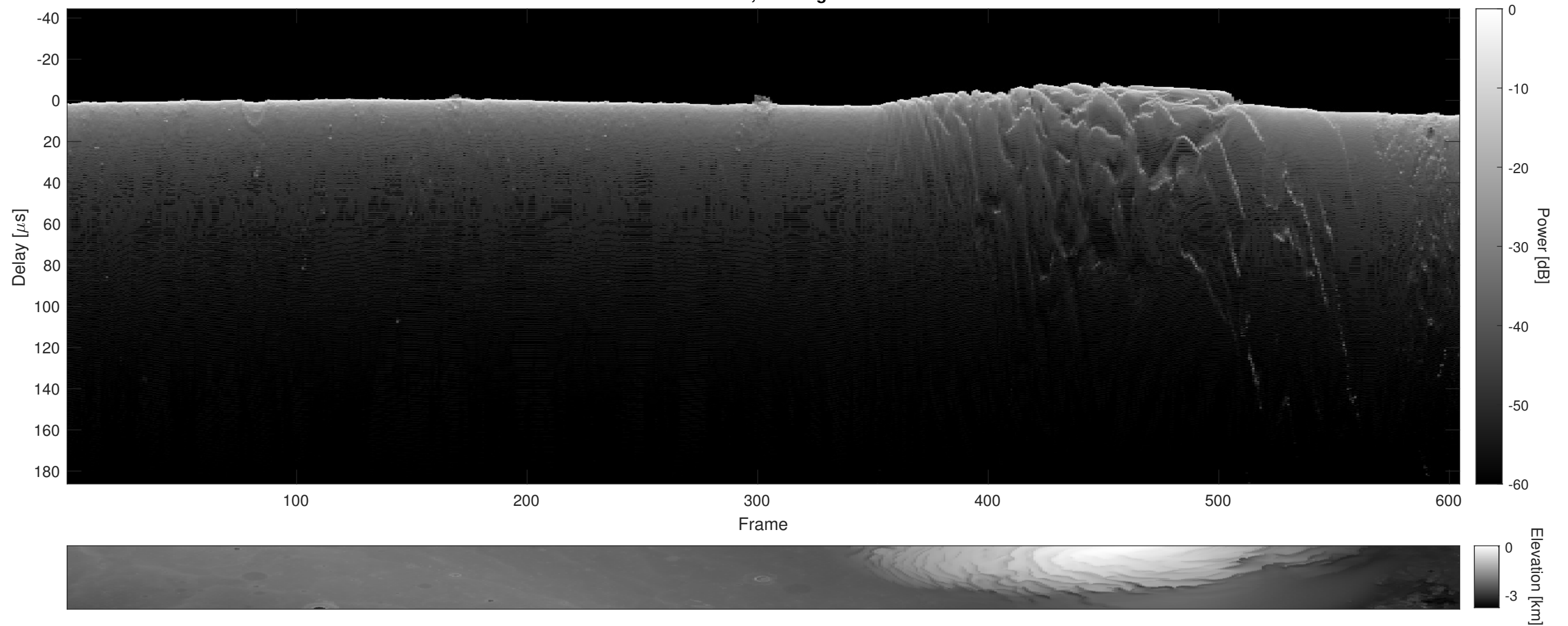
Orbit 5736, Cluttergram
