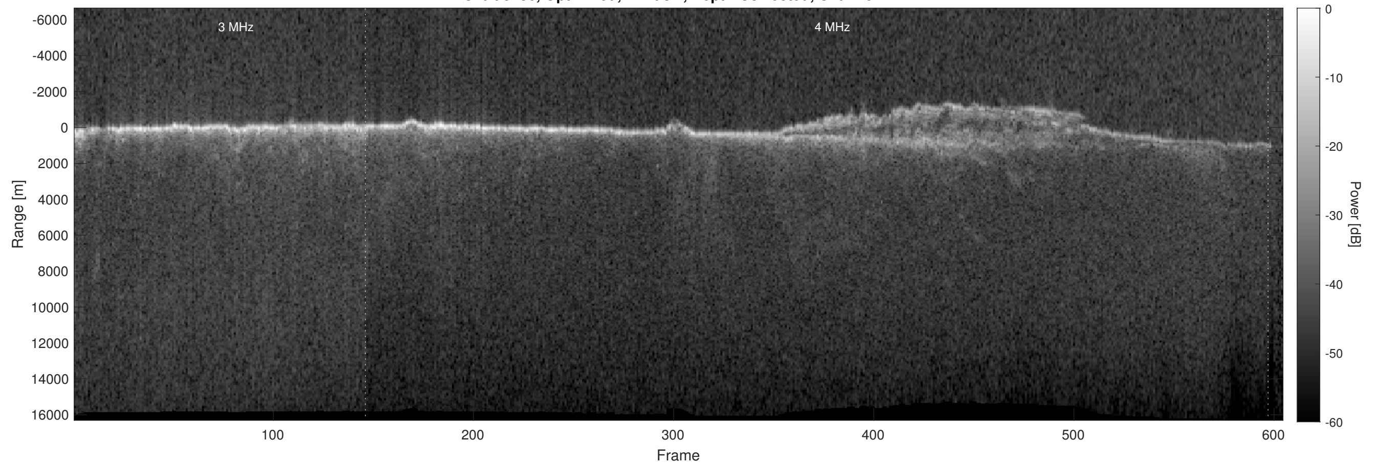
Orbit 5736, Optimized, Window, Depth-Corrected, Channel 2
