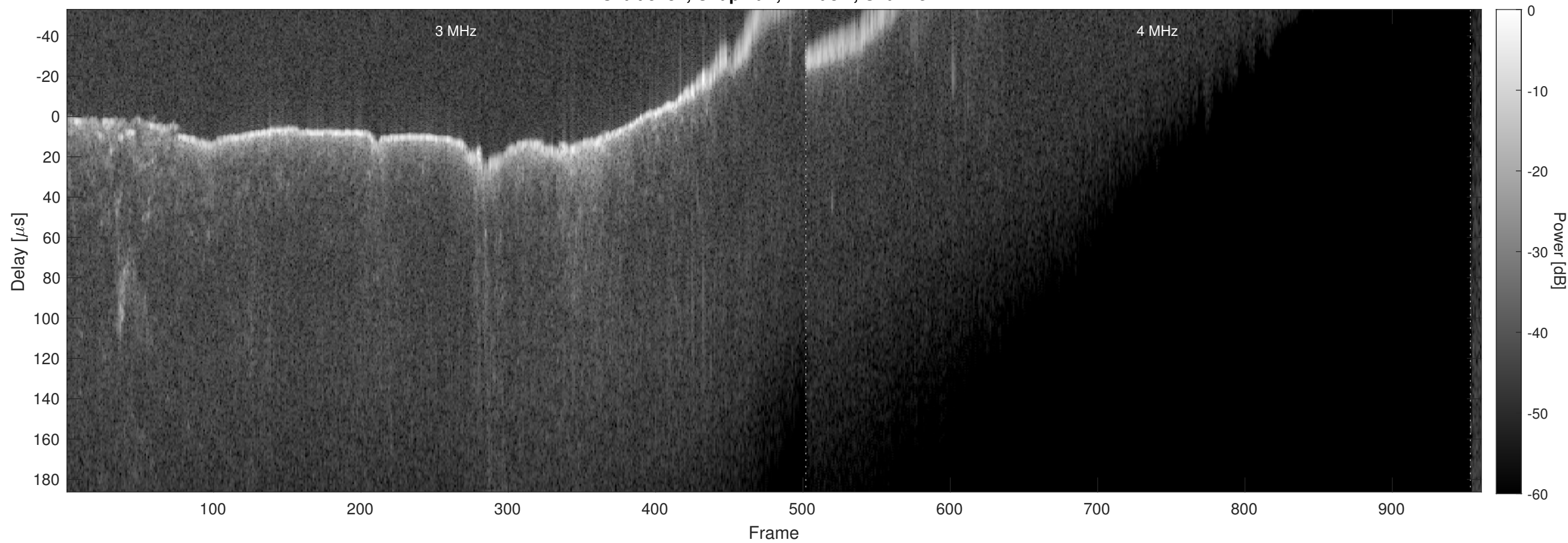
Orbit 5737, Chapman, Window, Channel 2
