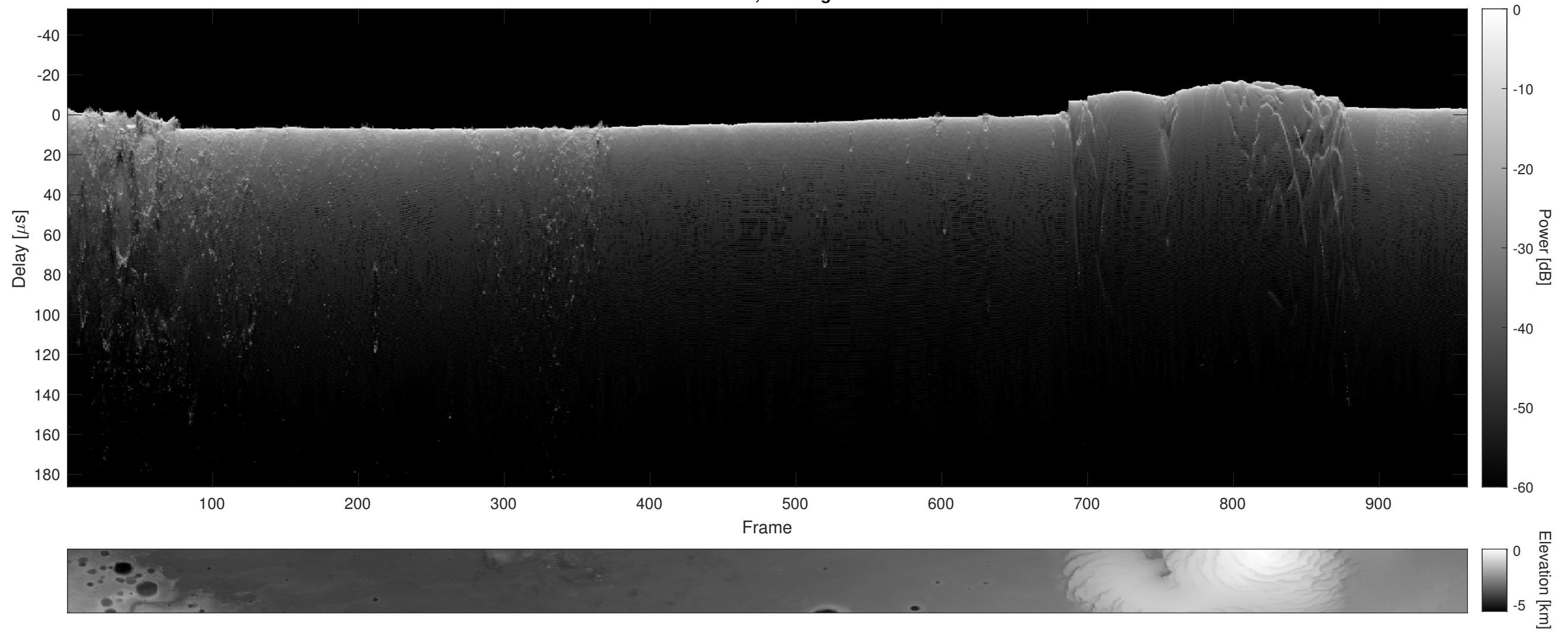
Orbit 5737, Cluttergram
