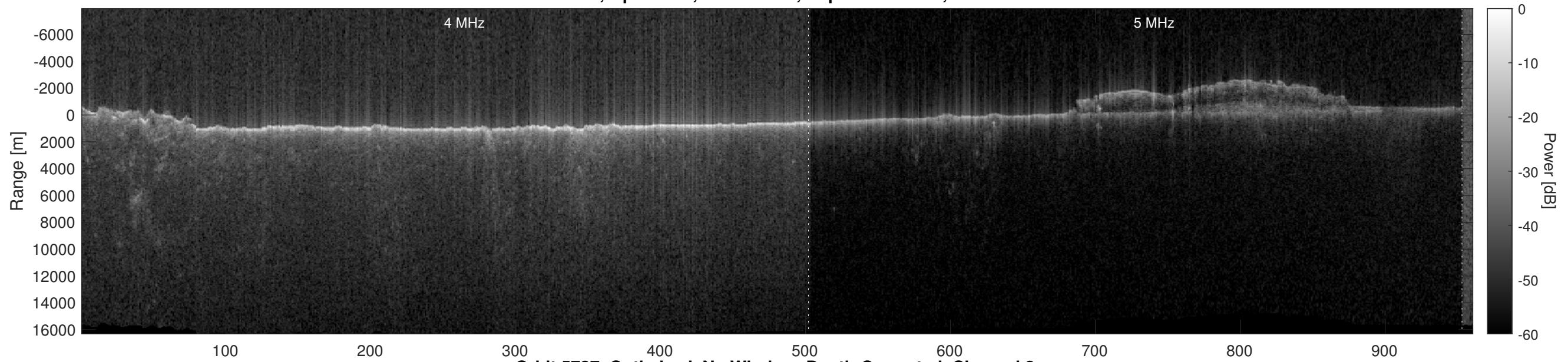
Orbit 5737, Optimized, No Window, Depth-Corrected, Channel 2
