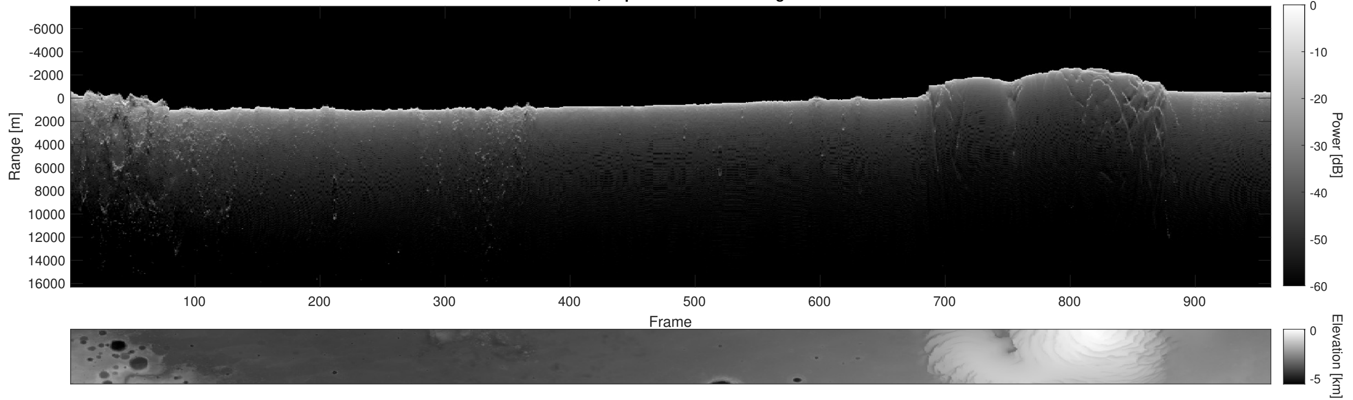
Orbit 5737, Depth-Corrected Cluttergram
