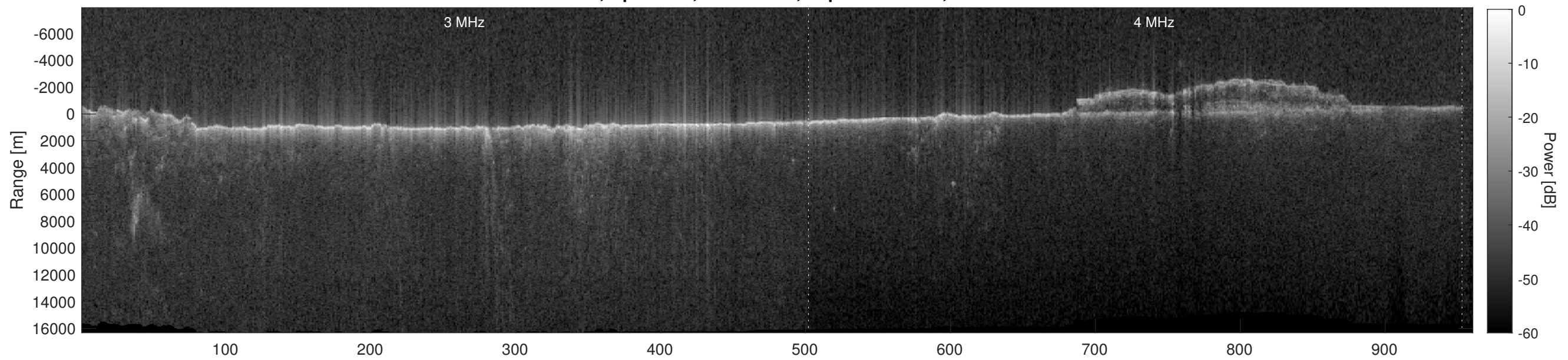
Orbit 5737, Depth-Corrected Cluttergram
