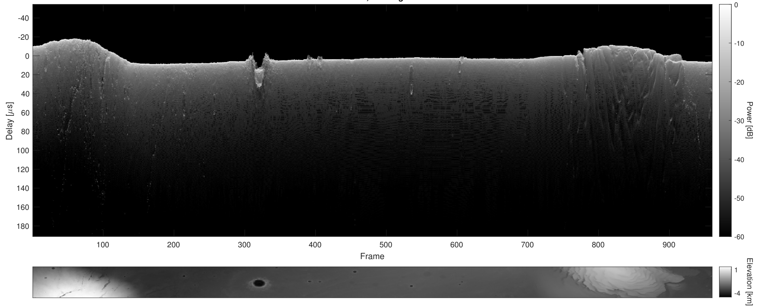
Orbit 5739, Cluttergram
