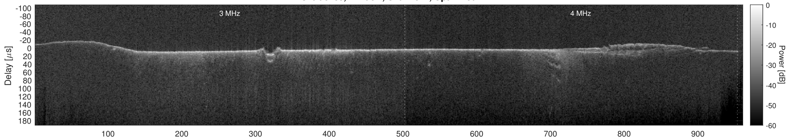
Orbit 5739, Cluttergram
