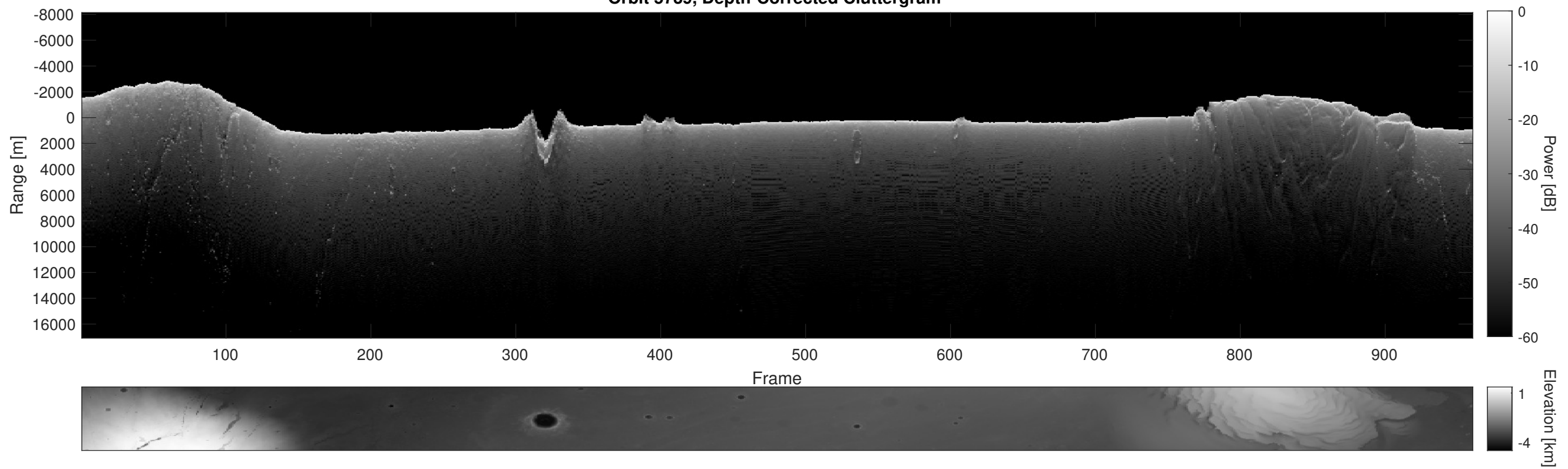
Orbit 5739, Depth-Corrected Cluttergram
