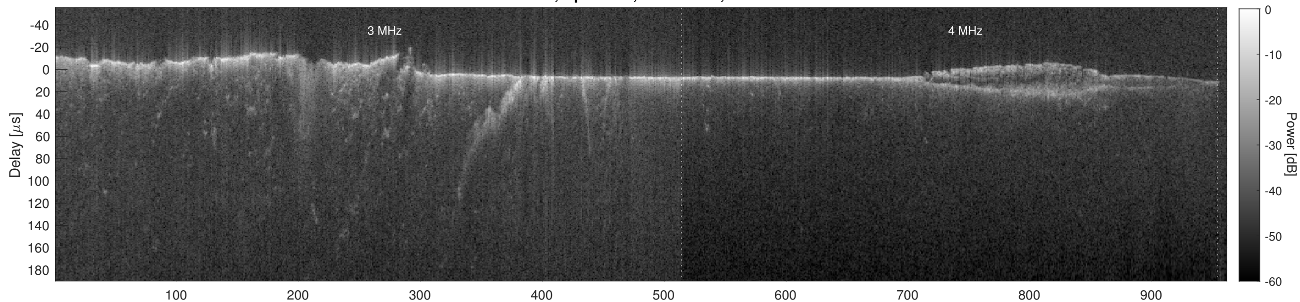
Orbit 5740, Cluttergram
