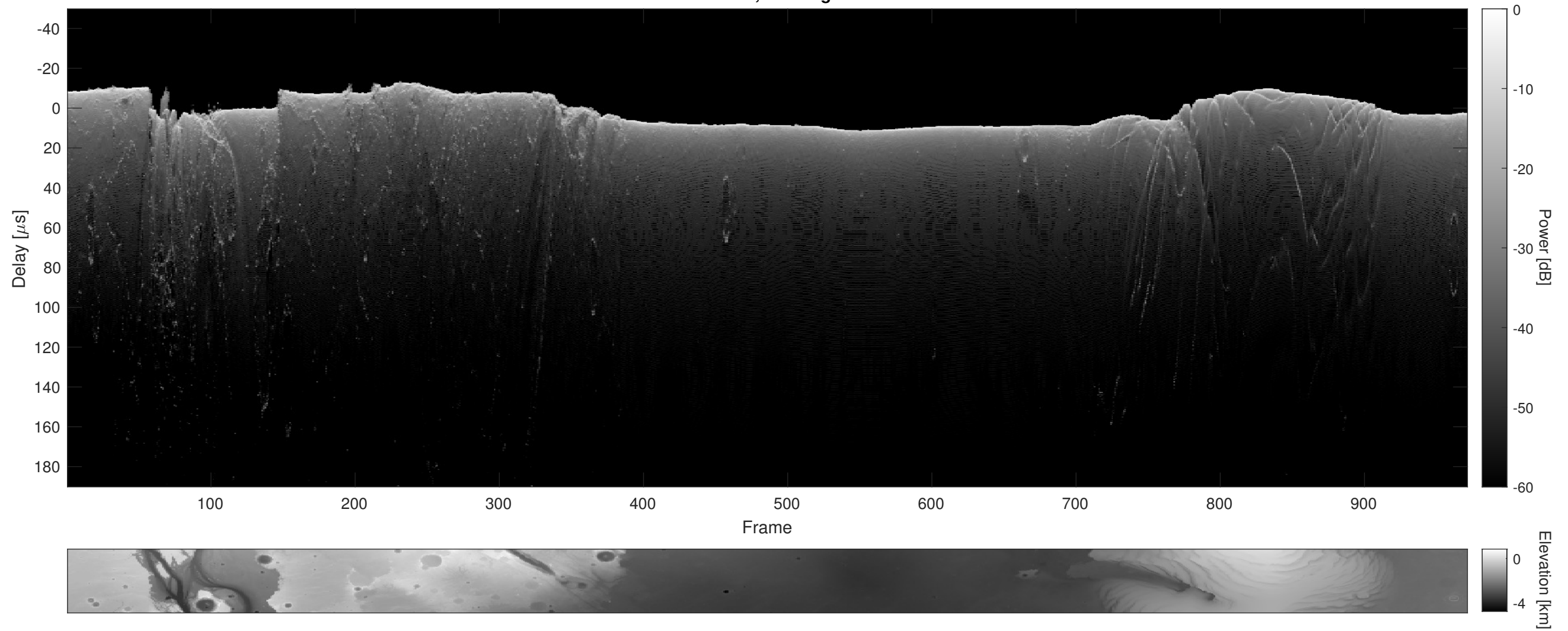
Orbit 5741, Cluttergram
