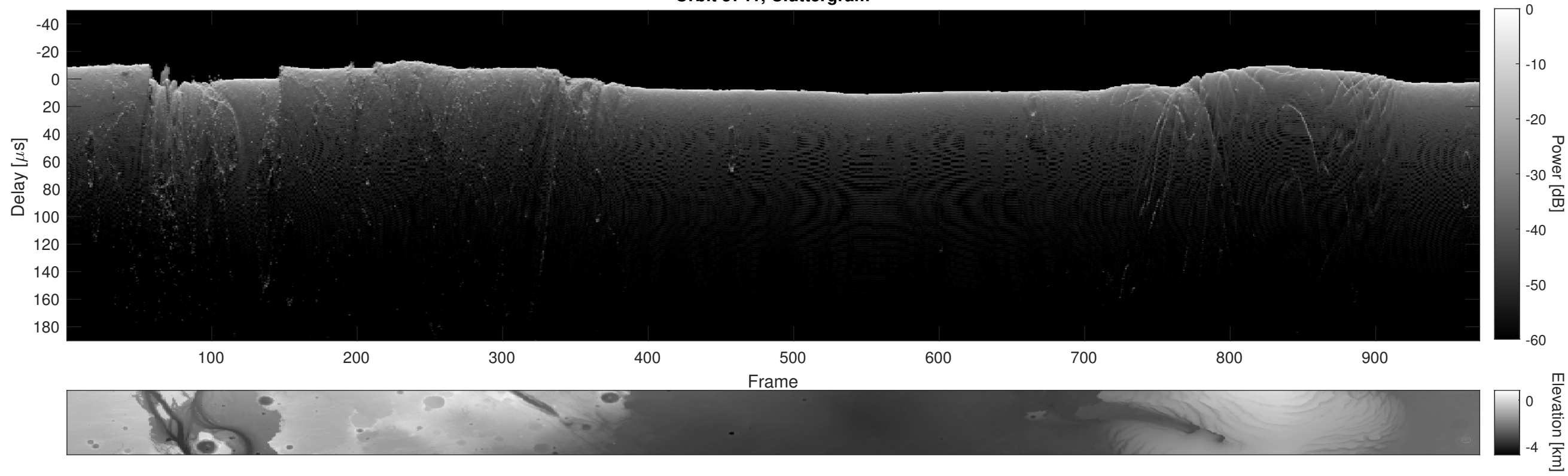
Orbit 5741, Cluttergram
