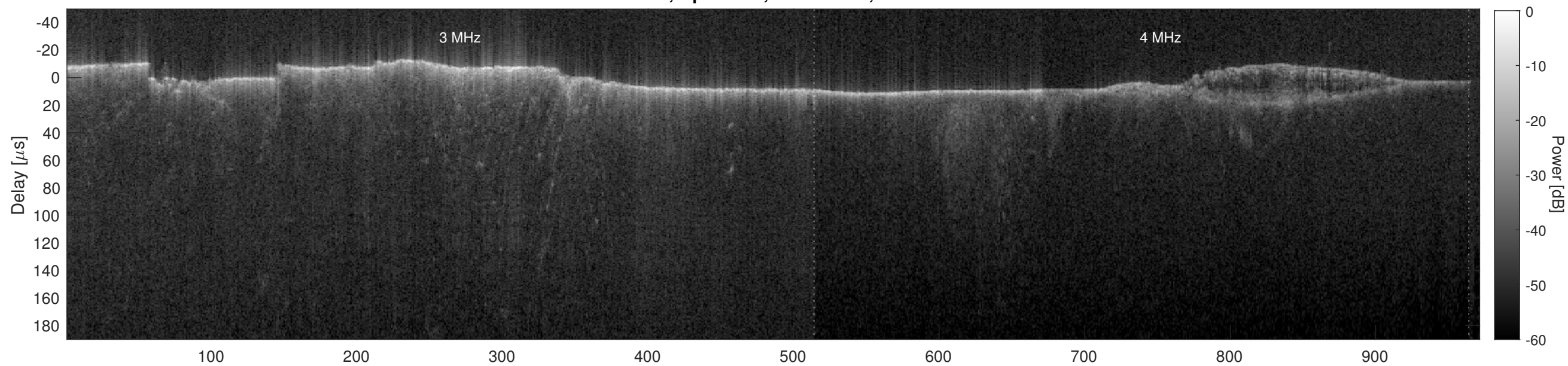
Orbit 5741, Cluttergram
