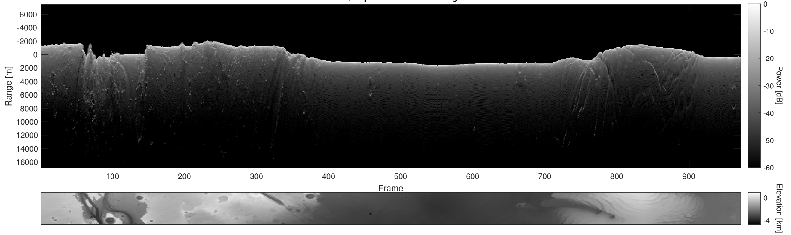
Orbit 5741, Depth-Corrected Cluttergram
