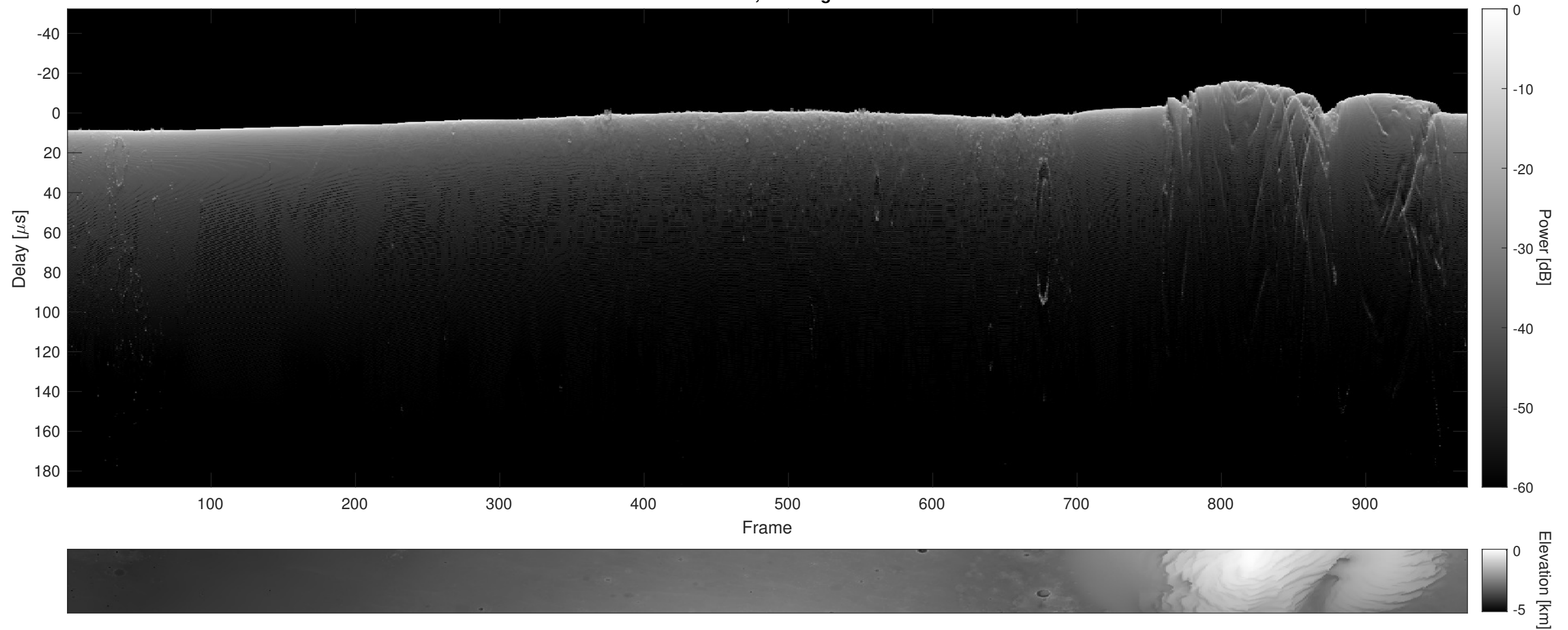
Orbit 5742, Cluttergram
