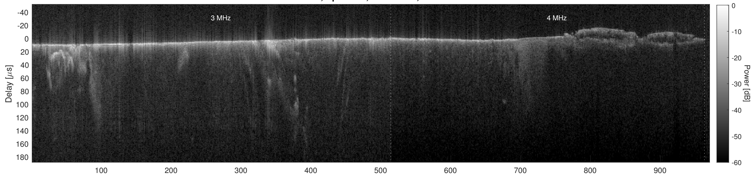
Orbit 5742, Cluttergram
