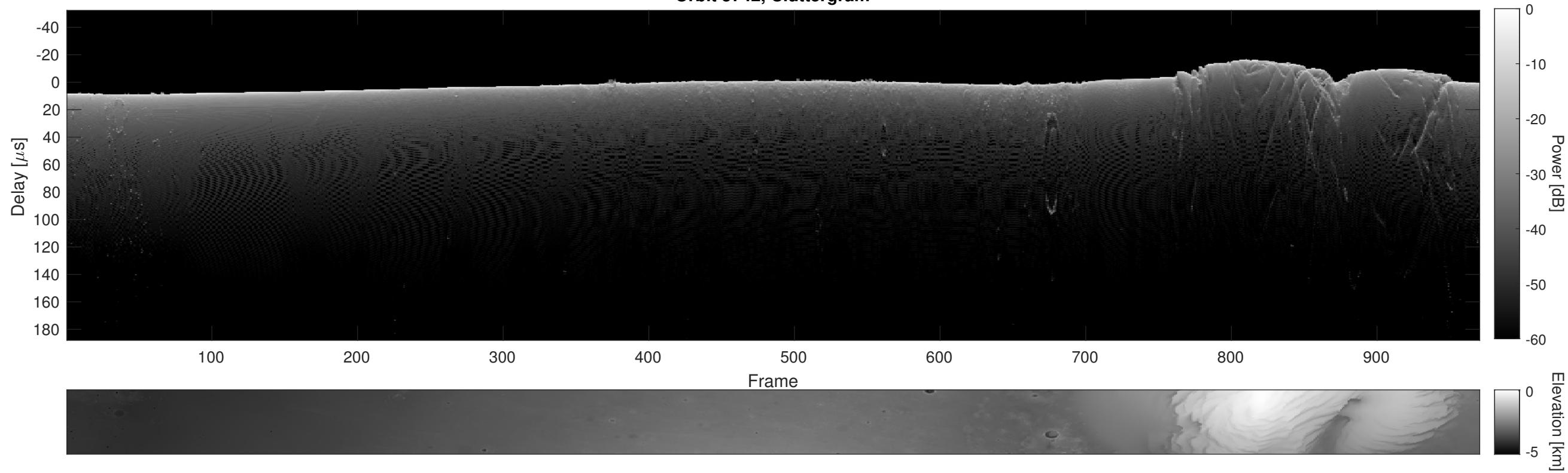
Orbit 5742, Cluttergram
