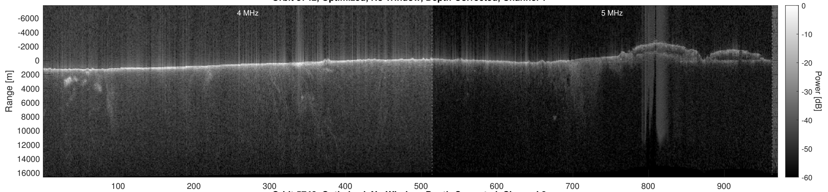
Orbit 5742, Optimized, No Window, Depth-Corrected, Channel 2
