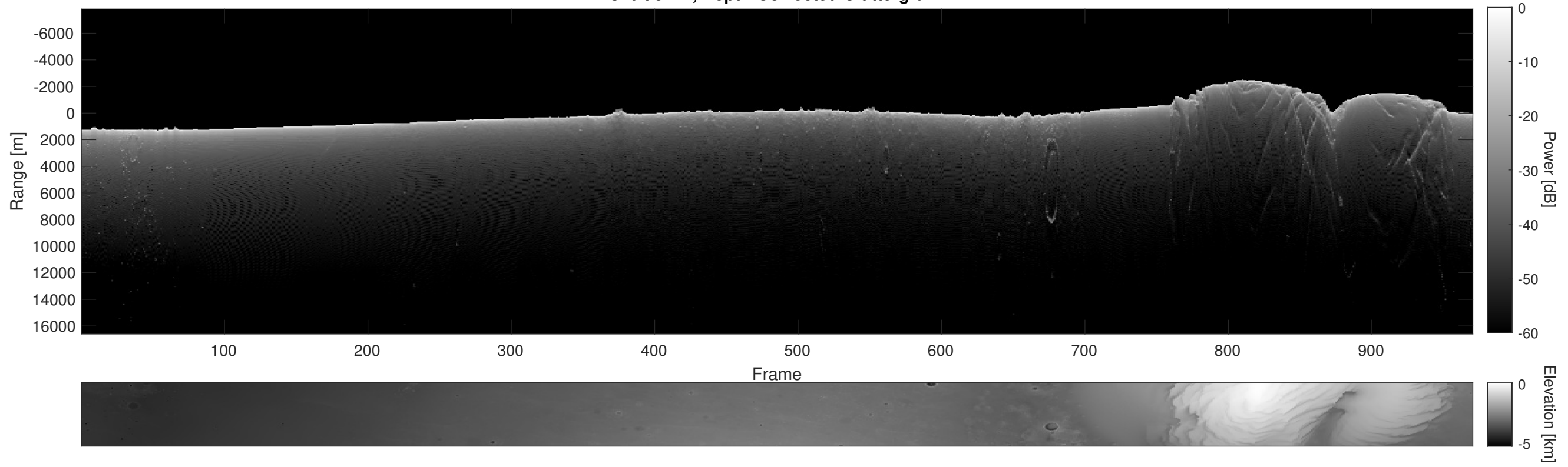
Orbit 5742, Depth-Corrected Cluttergram
