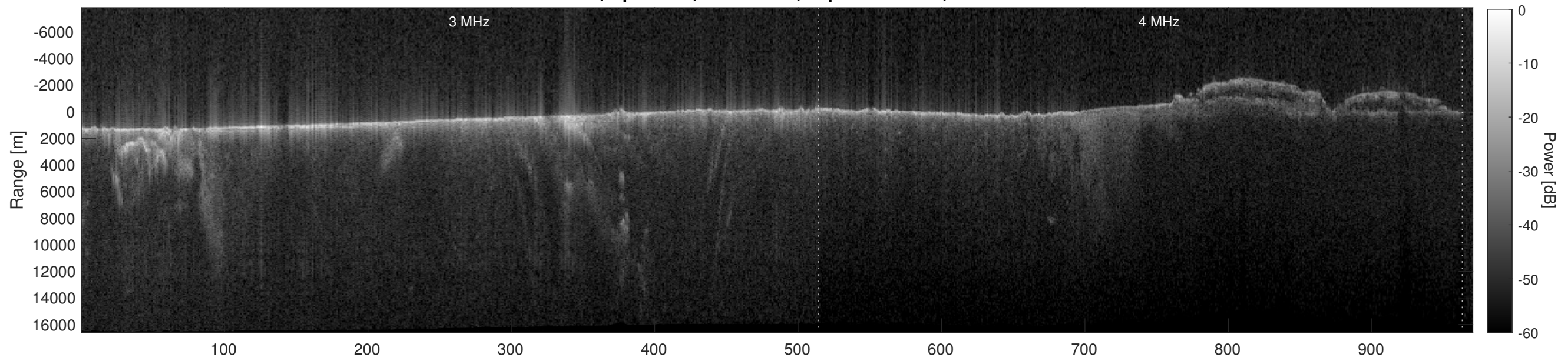
Orbit 5742, Depth-Corrected Cluttergram
