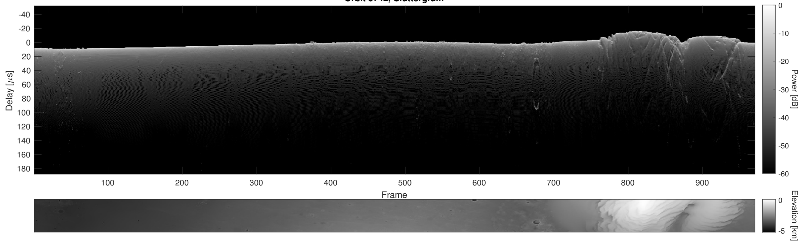
Orbit 5742, Cluttergram
