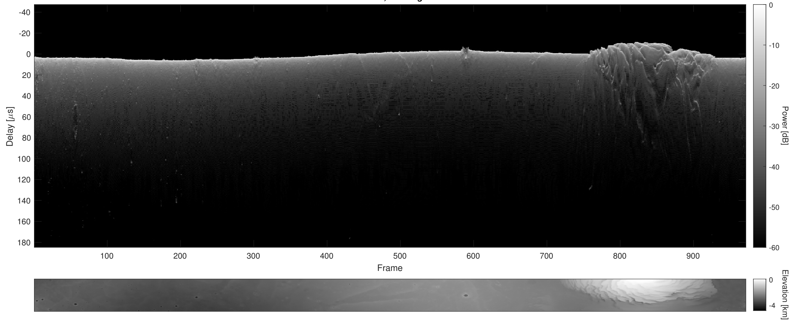
Orbit 5743, Cluttergram
