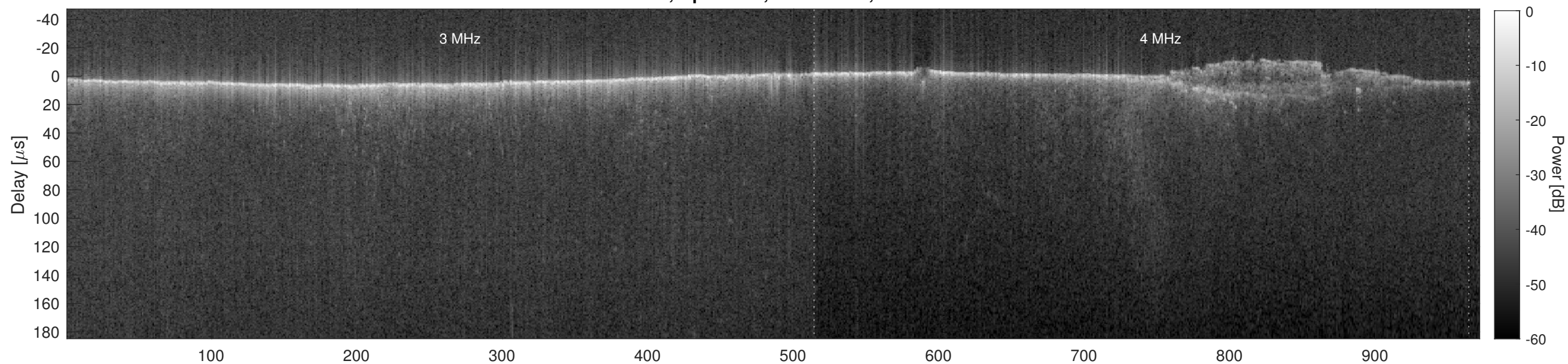
Orbit 5743, Cluttergram
