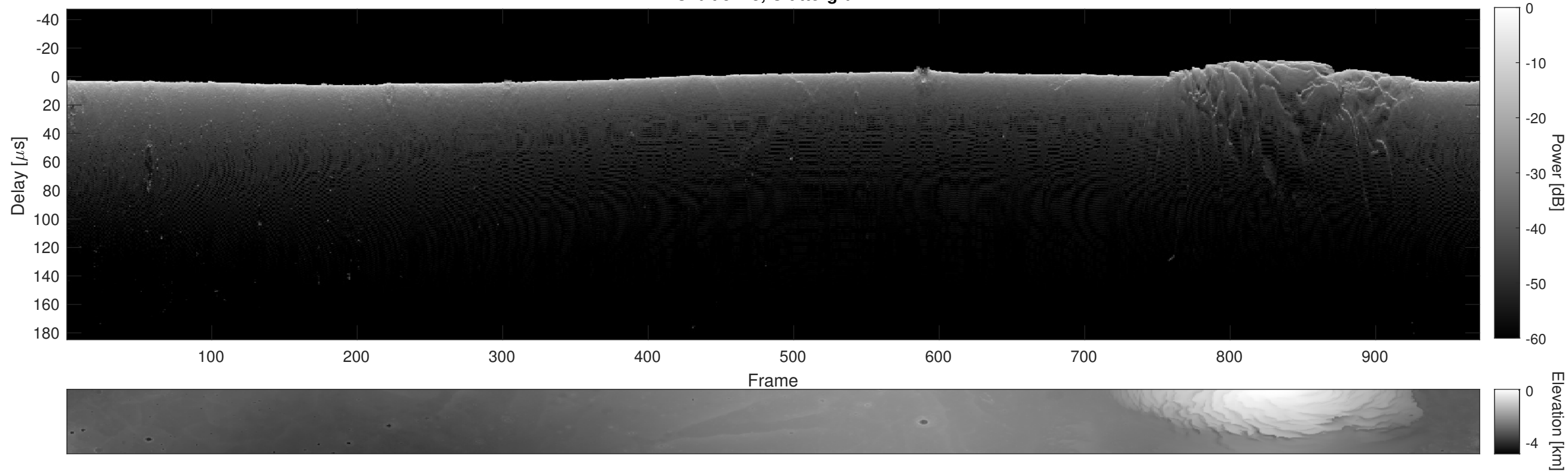
Orbit 5743, Cluttergram
