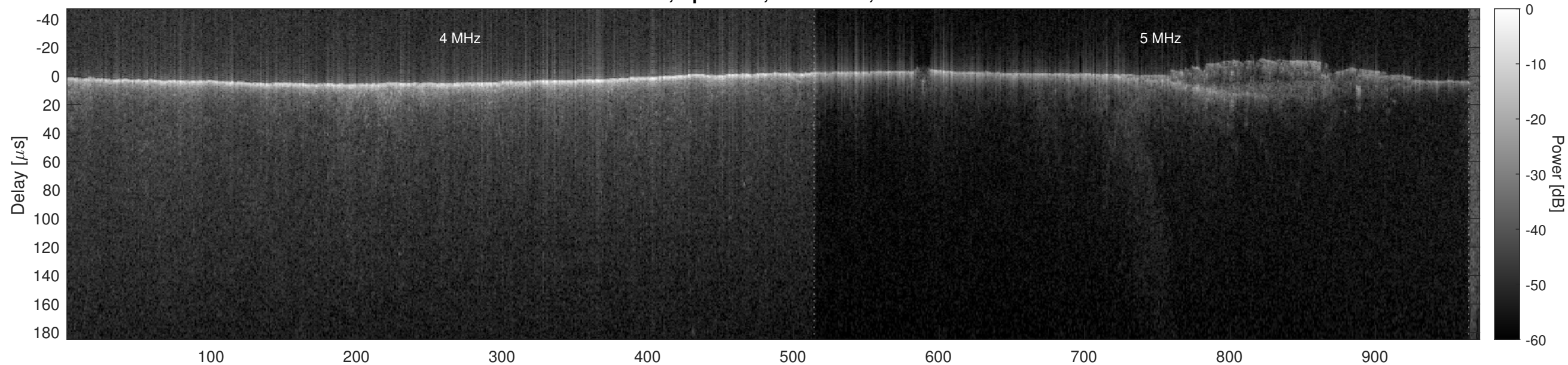
Orbit 5743, Optimized, No Window, Channel 2
