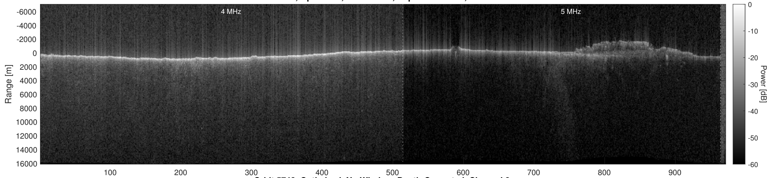
Orbit 5743, Optimized, No Window, Depth-Corrected, Channel 2
