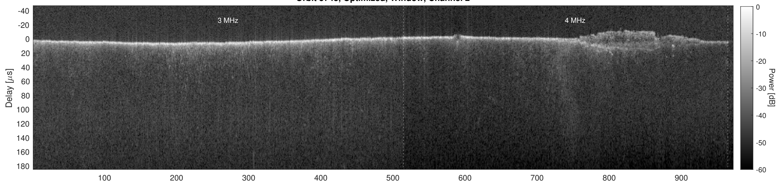
Orbit 5743, Cluttergram
