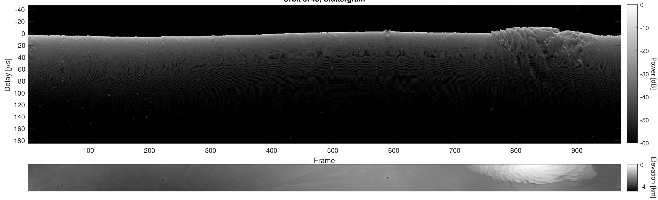
Orbit 5743, Cluttergram
