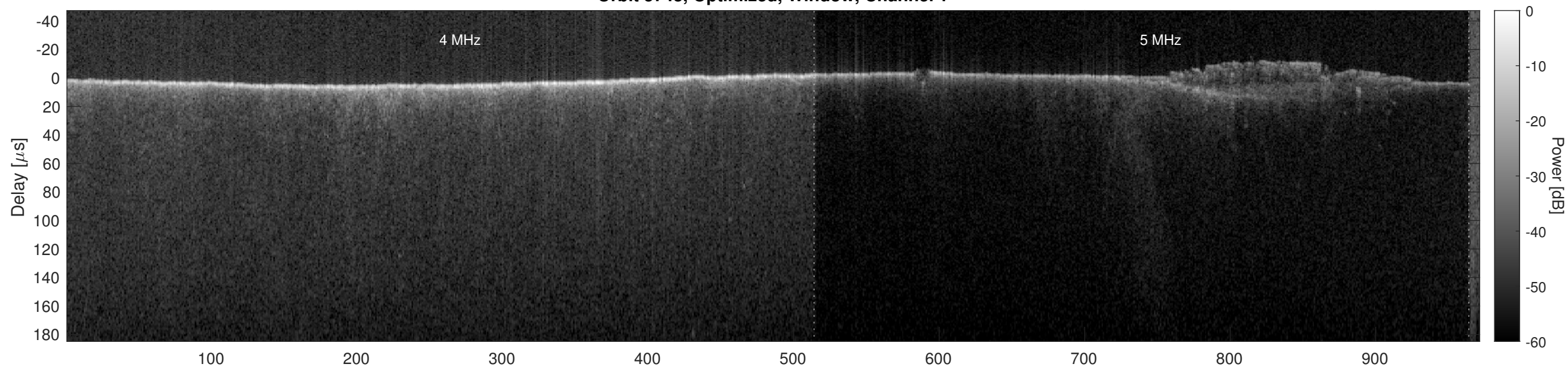
Orbit 5743, Optimized, Window, Channel 2
