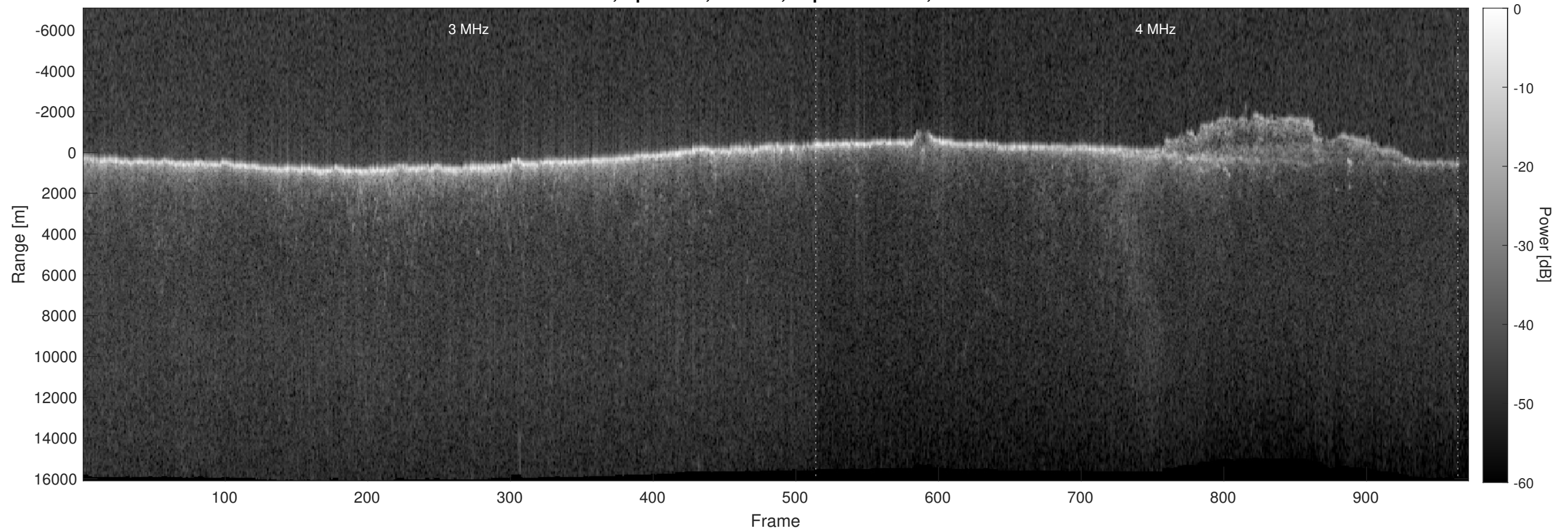
Orbit 5743, Optimized, Window, Depth-Corrected, Channel 2
