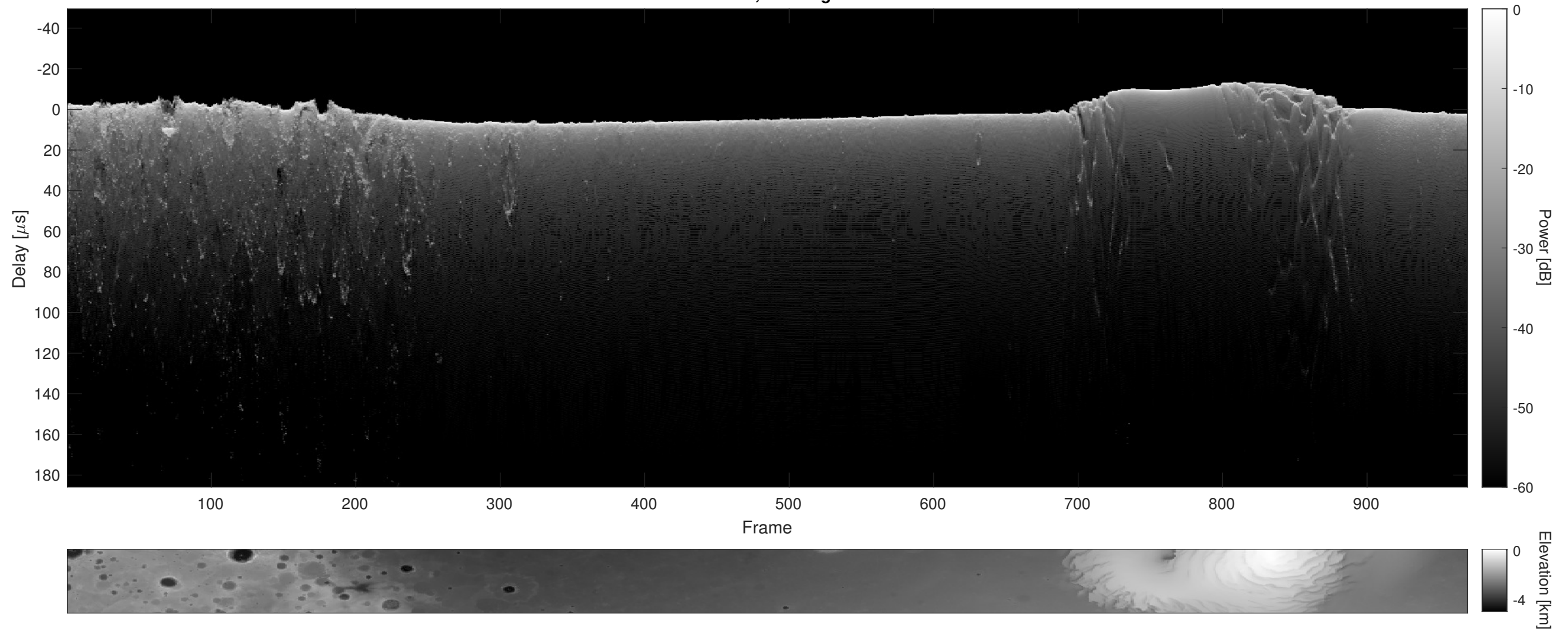
Orbit 5744, Cluttergram
