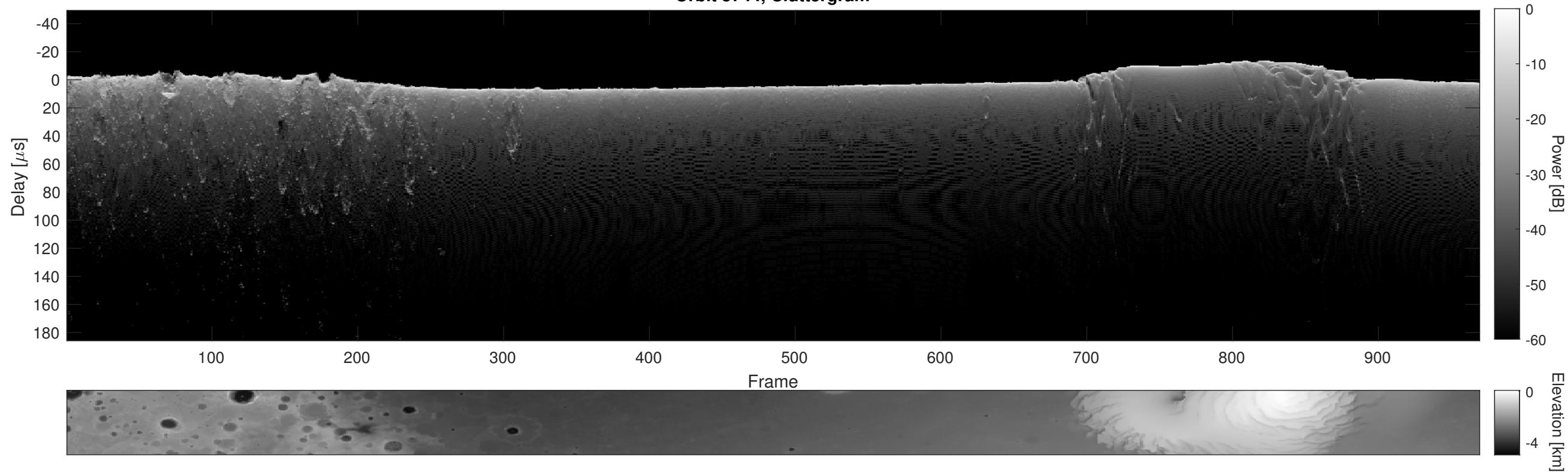
Orbit 5744, Cluttergram
