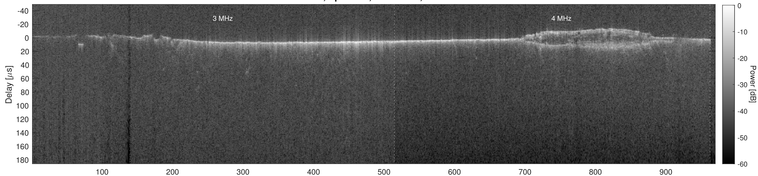
Orbit 5744, Cluttergram
