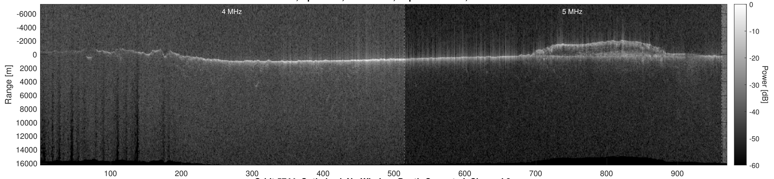
Orbit 5744, Optimized, No Window, Depth-Corrected, Channel 2
