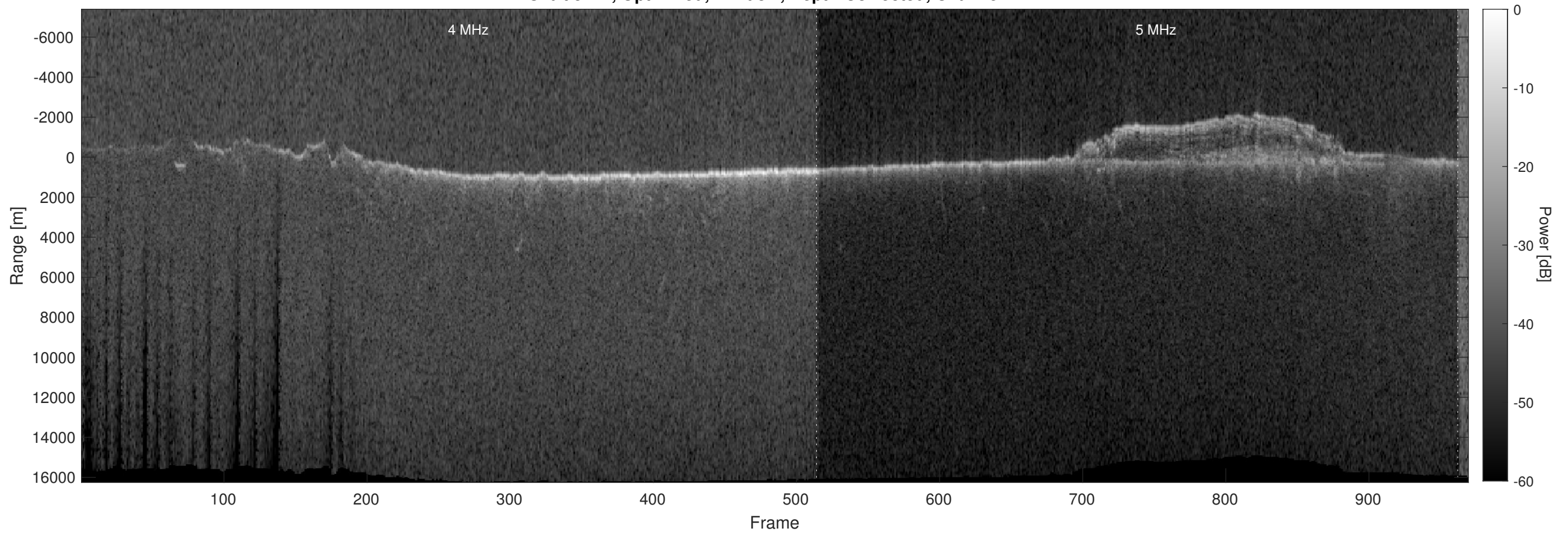
Orbit 5744, Optimized, Window, Depth-Corrected, Channel 2
