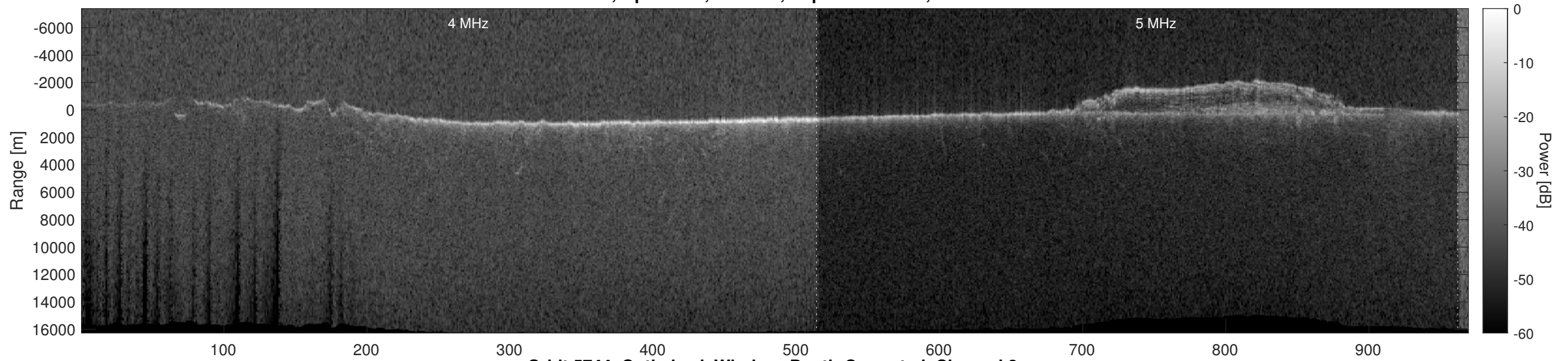
Orbit 5744, Optimized, Window, Depth-Corrected, Channel 2
