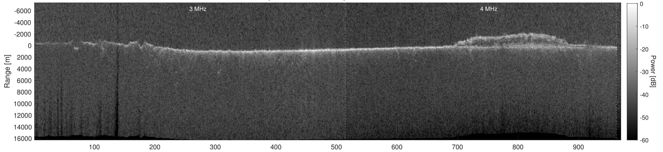
Orbit 5744, Depth-Corrected Cluttergram
