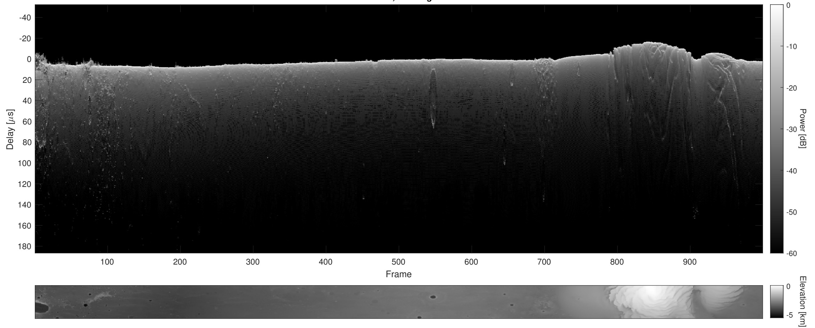
Orbit 5753, Cluttergram
