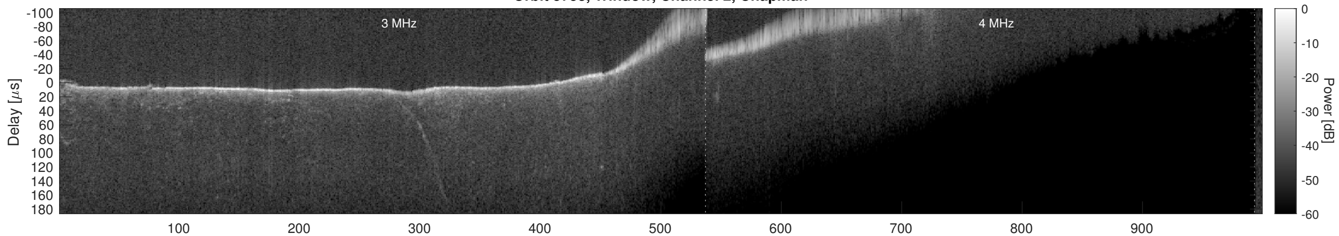
Orbit 5753, Window, Channel 2, Optimized
