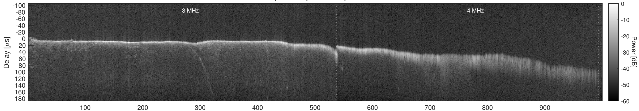
Orbit 5753, Window, Channel 2, Chapman
