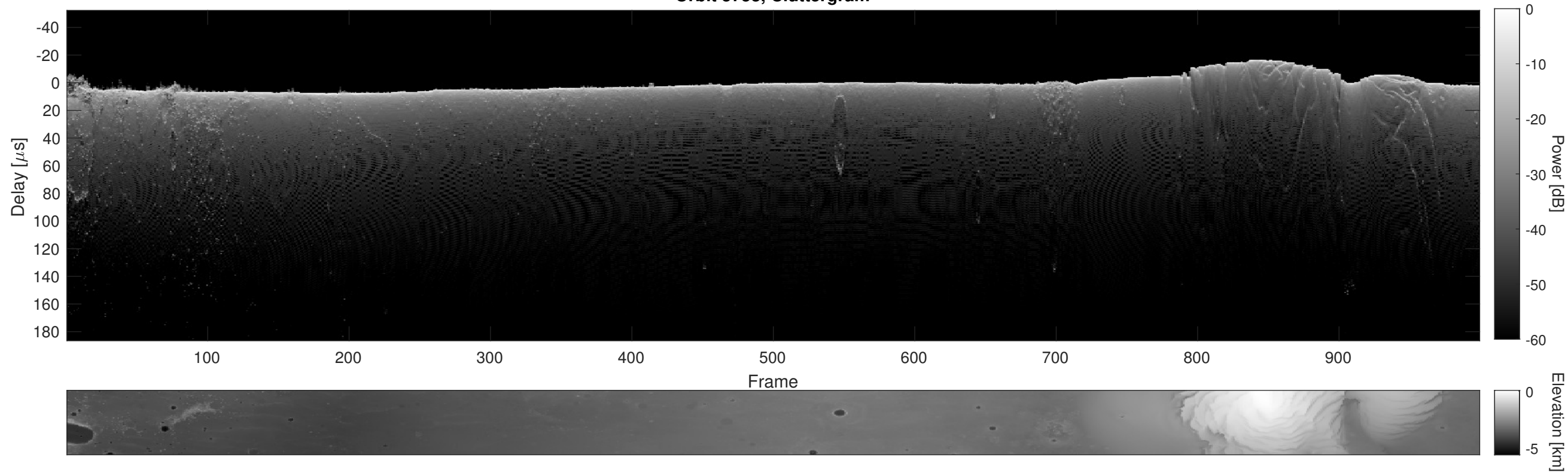
Orbit 5753, Cluttergram
