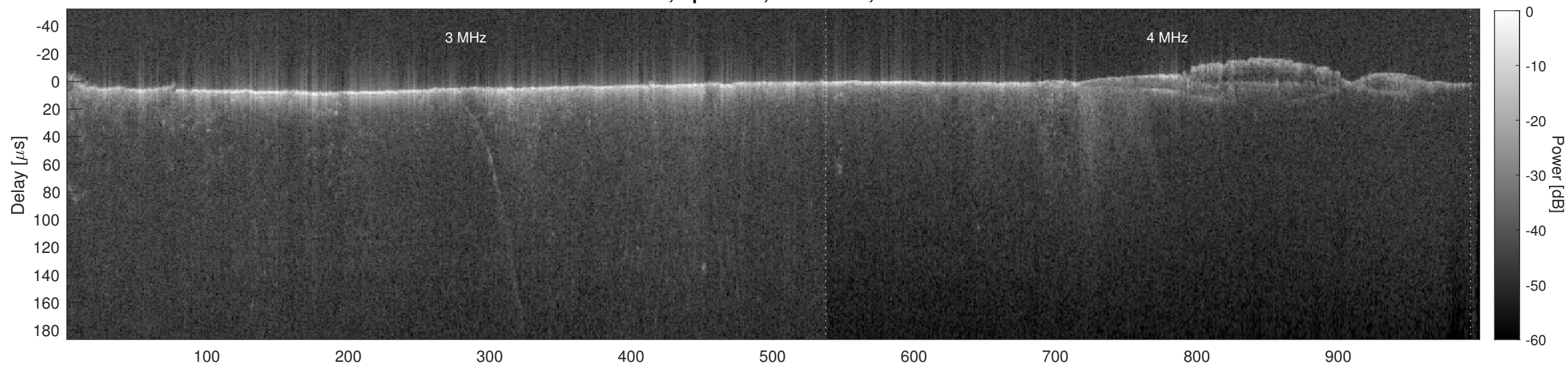
Orbit 5753, Cluttergram
