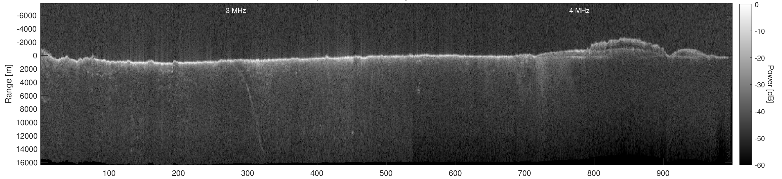
Orbit 5753, Depth-Corrected Cluttergram
