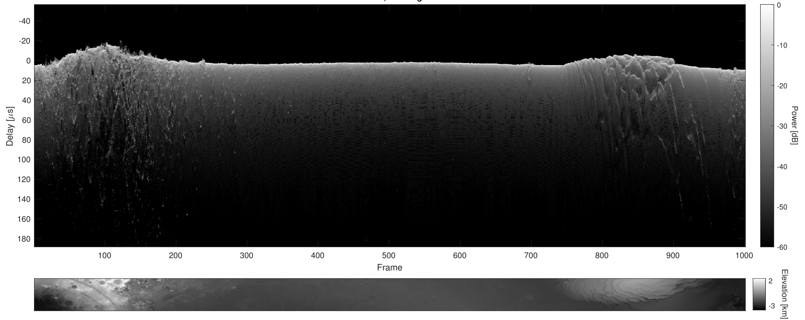
Orbit 5754, Cluttergram
