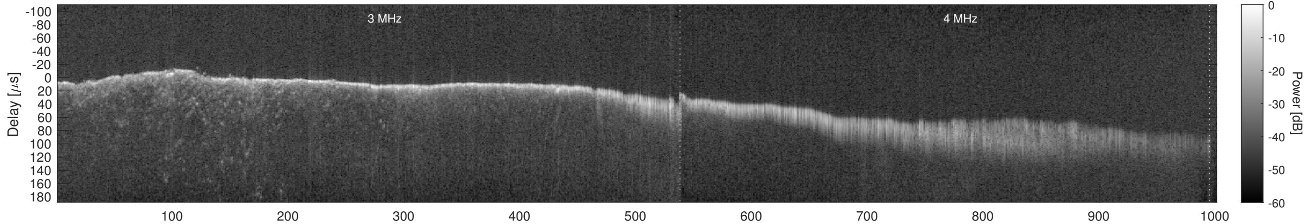
Orbit 5754, Window, Channel 2, Chapman
