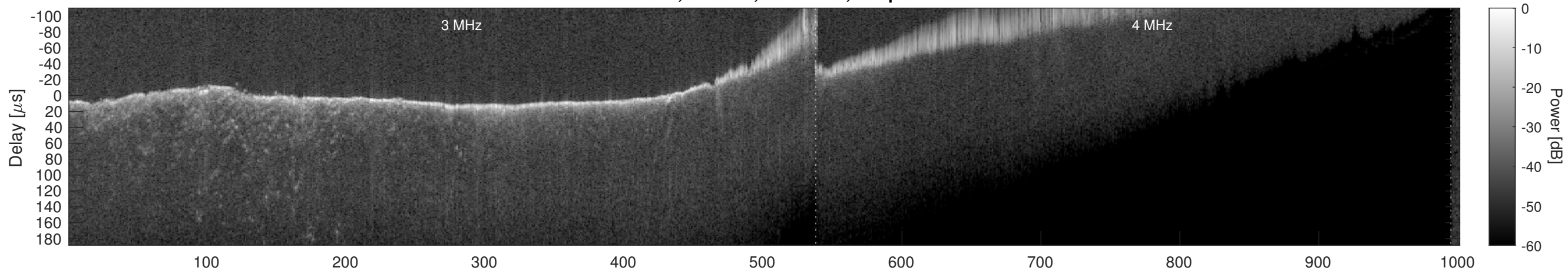
Orbit 5754, Window, Channel 2, Optimized
