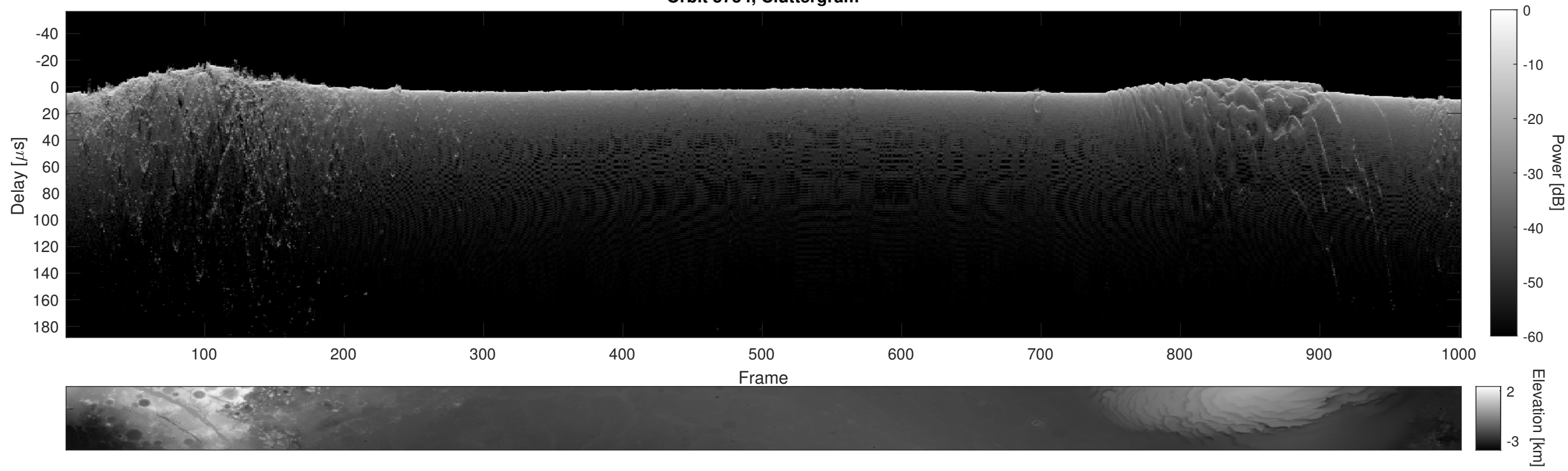
Orbit 5754, Cluttergram
